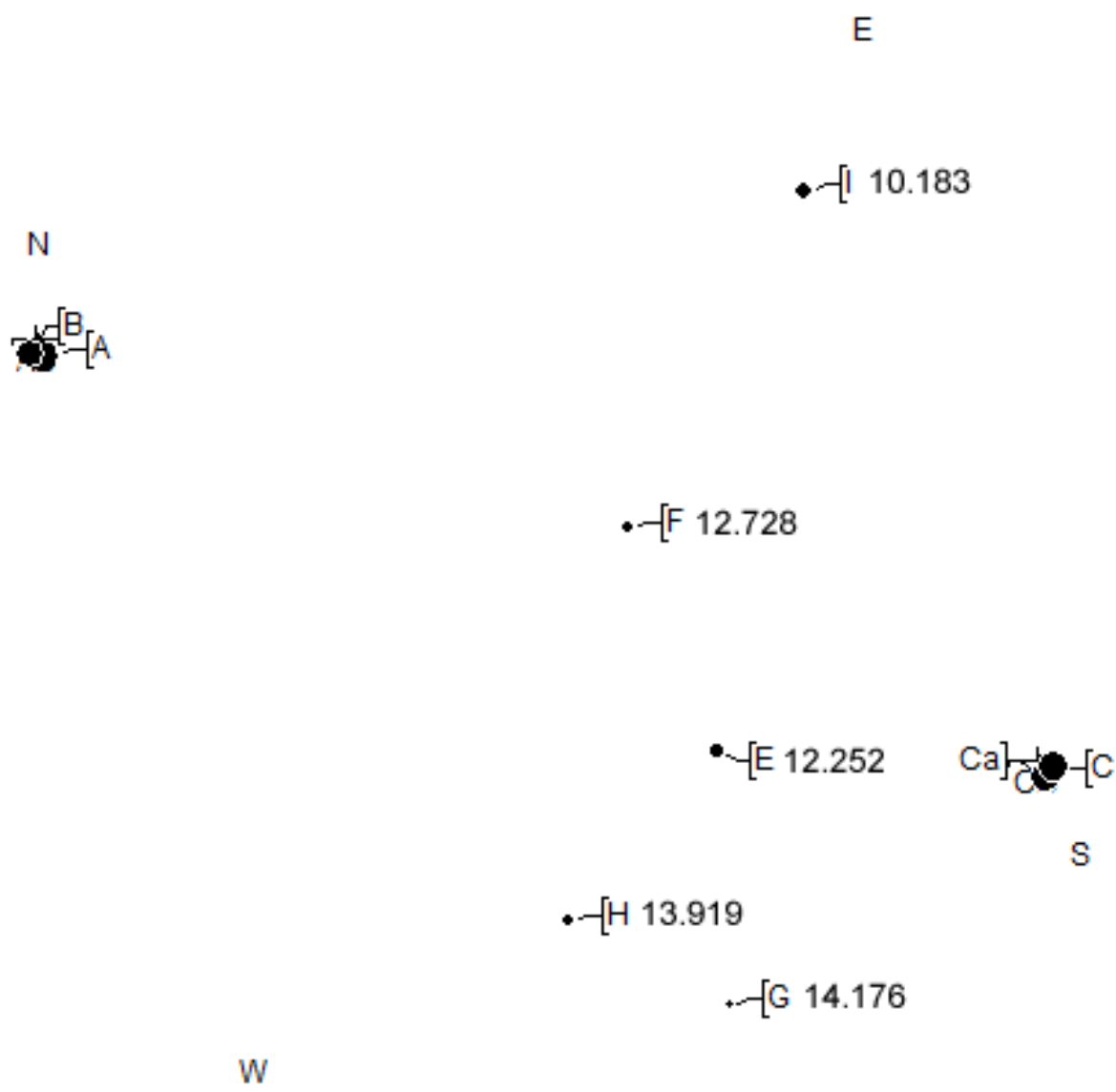
Eps Lyr Detail
